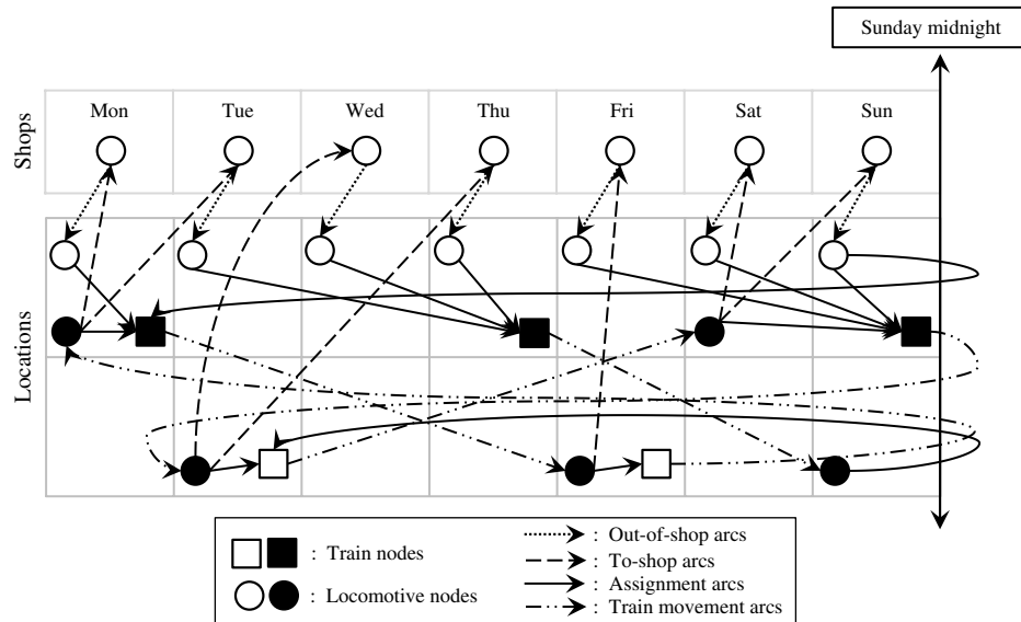
Figure 2 Network Representation of the Single Commodity Planning Model
