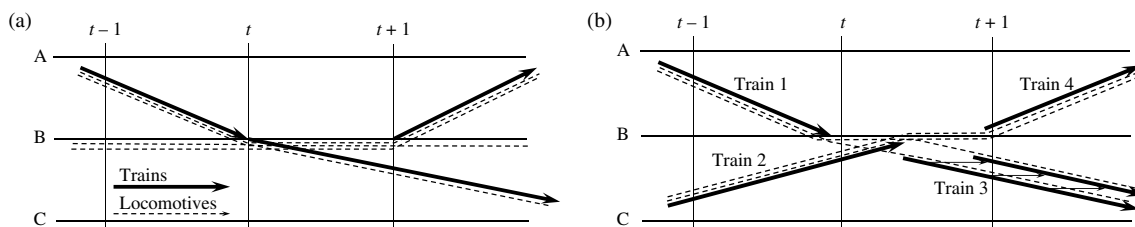
Figure 1 Illustration of a Classical Time-Space Network for Multicommodity Flow Problems (a), and a Task-Graph Network That Provides for Continuous Arrival and Departure Times (b)
