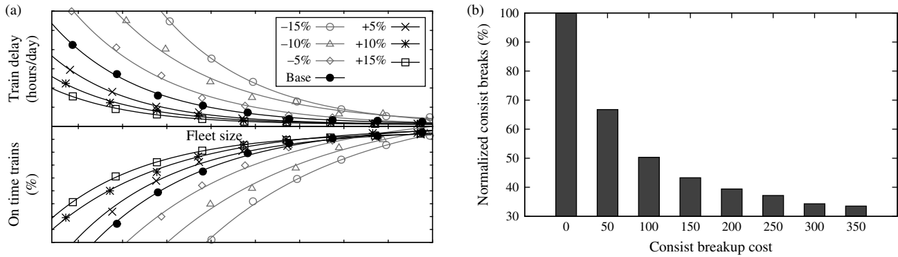
Figure 12 (a) On-Time Trains and Train Delay, as a Function of Fleet Size, for a Range of Average Train Speeds; (b) Consist Breakups for Different Consist Breakup Costs, Normalized as a Percent of Consist Breakups When the Cost Is Zero
