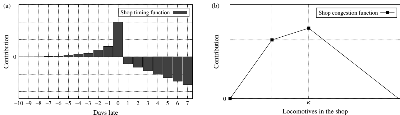
Figure 8 (a) Contribution for Arriving to Shop as a Function of the Arrival Time Relative to the Scheduled Arrival Time, and (b) Shop Congestion Function, Showing Increasing Value Up to the Capacity of the Shop, Followed by a Downward Sloping Function If the Number of Locomotives Exceeds Capacity, Implying Queueing
