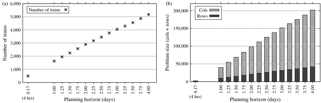
Figure 3 Size of the Integer Programming Model as a Function of the Planning Horizon
