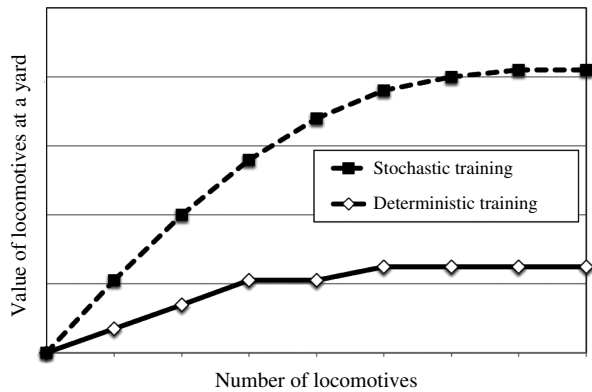
Figure 14 Deterministically and Stochastically Trained Value Function Approximations, for a Particular Yard at a Point in Time in the Norfolk Southern Network
