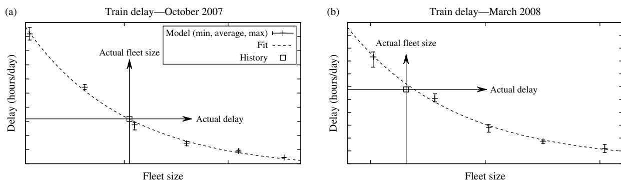
Figure 11 Train Delay as a Function of Fleet Size, Compared to Historical Delay for October 2007 (Used for Calibration) and March 2008
