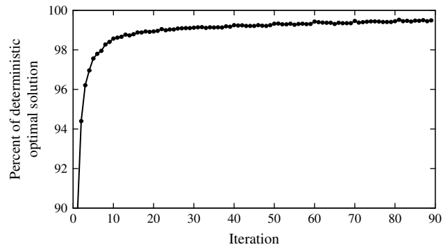
Figure 7 The ADP Objective Function as a Percent of the Optimal Deterministic Solution Obtained Using CPLEX, for a Problem with a 3.5 Day Planning Horizon
