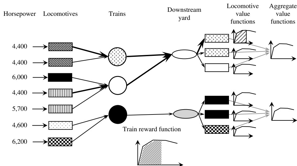
Figure 5 Illustration of Locomotive Assignment Policy Using Hierarchical Value Function Approximations
