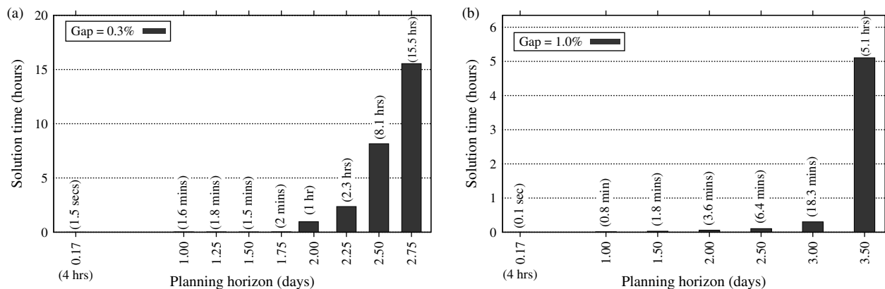
Figure 4 CPU Time for Integer Programming Model as a Function of the Planning Horizon
