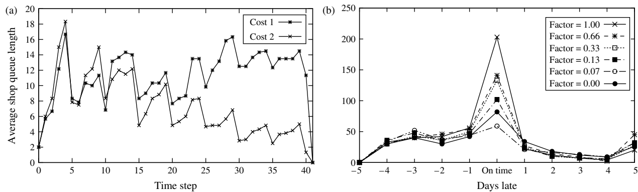
Figure 13 Effect of the Congestion Cost on the Shop Queue (a), and the Effect of the Penalty Cost on Arrival Times to Shop (b)
